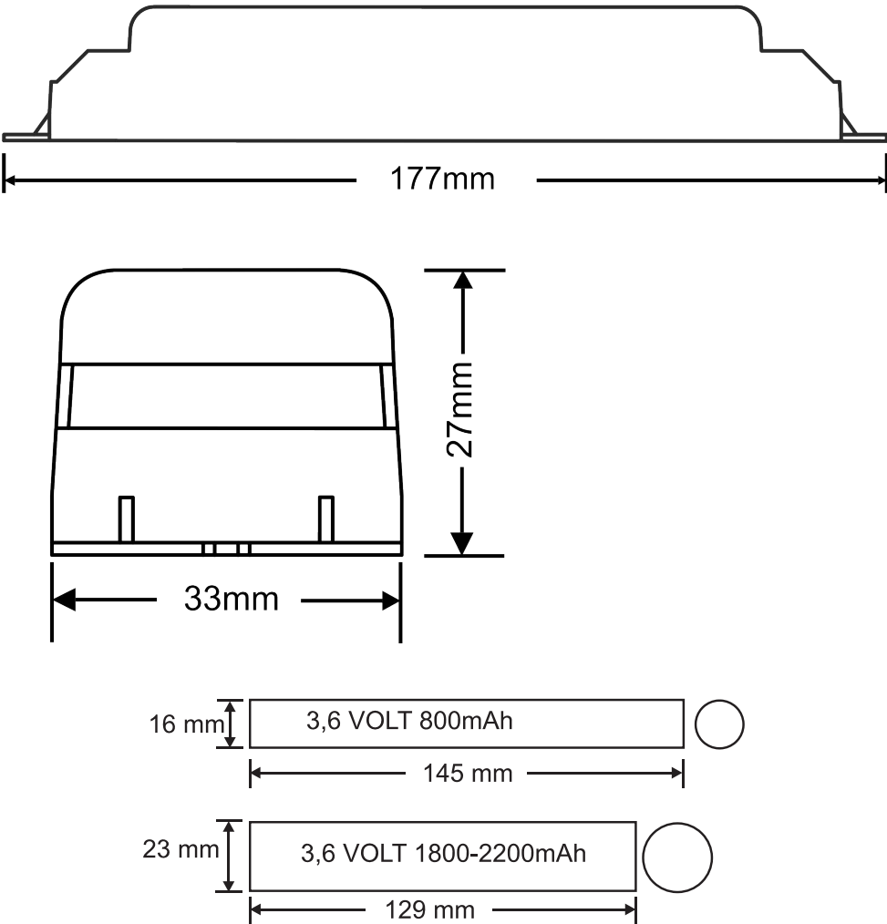
AK-3300 BATTERIES
